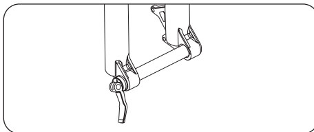
Quick-release axle in the fork dropouts, without hub, Rock Shox® fork
