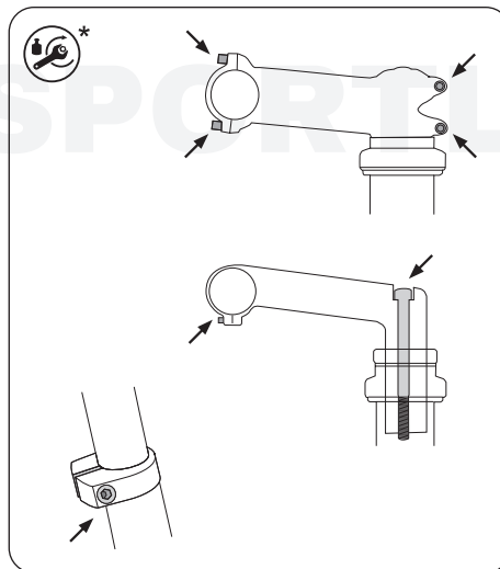
Possible positions for adjusting bolted connections
